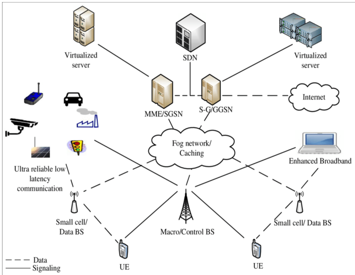
Fig. 1: General Architecture of 5G Wireless System
