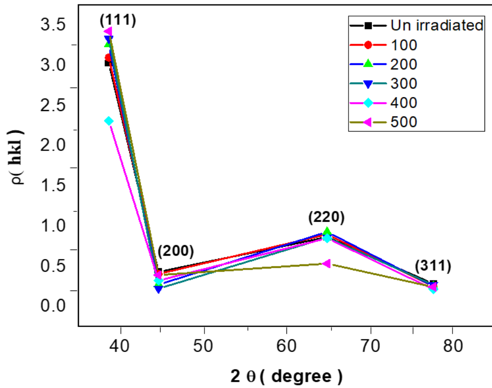
Fig. 4: Texture coefficients (hkl) as a function of 2Θ for a given laser shot
